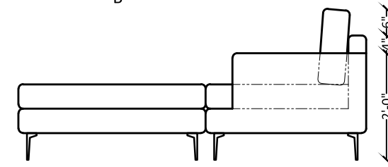
SIDE ELEVATION-D
